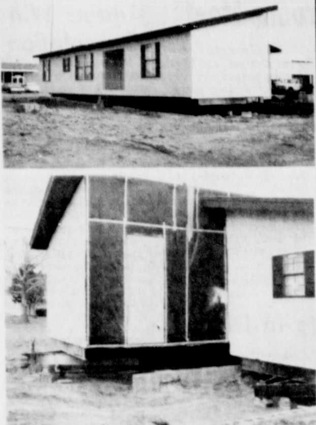
This new modular home owned by Mr. and Mrs. E.J. Windom Sr., was moved onto the corner of 2nd and Commerce last week. The three-bedroom, manufactured home was built in sections, then brought to McLean, with the final construction being done at the homestead. The Childress company which built the house recently supplied more than 200 housing and support units to a firm in Algeria. The homes reportedly were to be used as housing for El Paso Natural Gas Company employees who recently were transferred from the United States to Algeria for a two-year stay. (Staff Photos)
