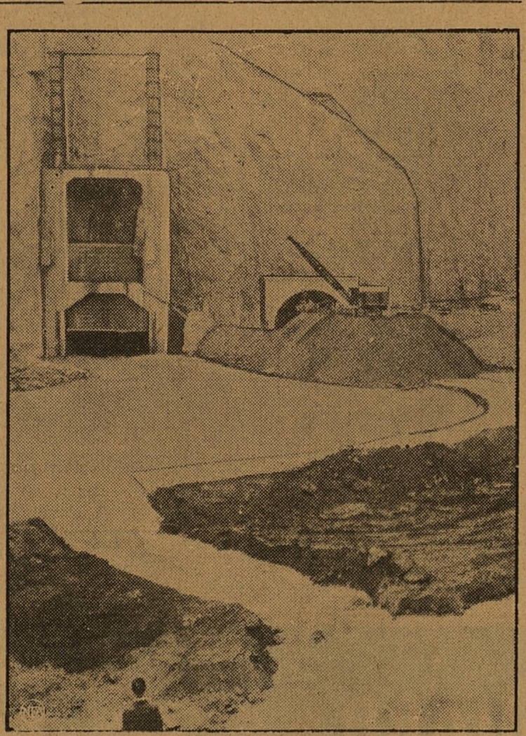
Man's control over the mighty Colorado river became reality when water poured down the spillway from No. 1 diversion tunnel to begin filling the mammoth reservoir of $49,000,000 Boulder dam. In this picture the gigantic bulkhead gate of No. 4 tunnel was being closed at the rate of nine inches a minute to divert the water to No. 1 tunnel, where control gates direct the flow.
