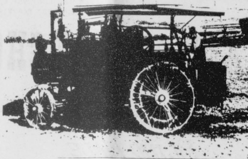
Photo is of a 1925 Russell steam engine. 20 horsepower. Owned by Bud Battin of Perryton; the engineer is Homer Coverdale, Perryton.
