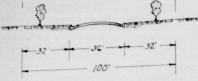
PAVING PLAN BETWEEN VIRGINIA & BURLESON STS. ON SOUTH MAIN ST.
