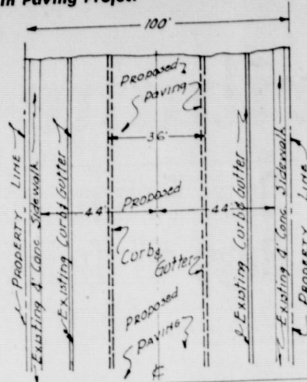
PAVING PLAN BETWEEN VIRGINIA & BURLESON STS. ON SOUTH MAIN ST.
