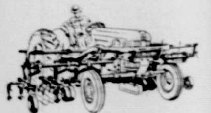
MF 141 4-Row Cultivator. One man can mount it in a couple of minutes. Adjusts for 28 to 42 in. row spacing. Rear gangs on 3-point hitch break to tire tracks.
