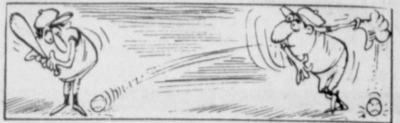
If one baseball is tossed horizontally while at the same instant a second baseball is dropped vertically from the same height, both of them will reach the ground simultaneously.
