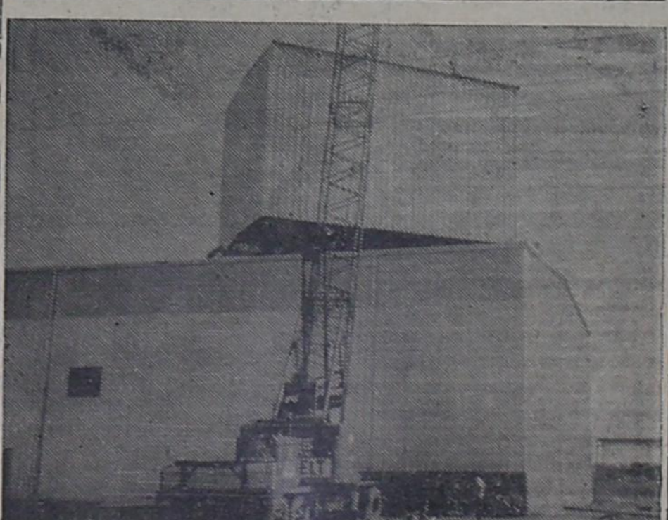
TOPPING OFF SHELLING PLANT — On Nov. 1, 1974, Gorman Peanut Co. set the all-steel building pictured here on top of the company's new shelling plant at Comyn, Texas. The building lifted weighs 26,000 pounds and is 40 feet long, 28 feet wide, and 24 feet high. The 130 foot crane was supplied by Minnis Erection Co. of Ft Worth. The building lifted will house equipment for grading shelled peanuts into various sizes. Gorman Peanut Co. expects to begin shelling peanuts soon and is presently drying, cleaning, buying, and storing all segregations of Spanish and Florunner farmer stock peanuts at Comyn.
