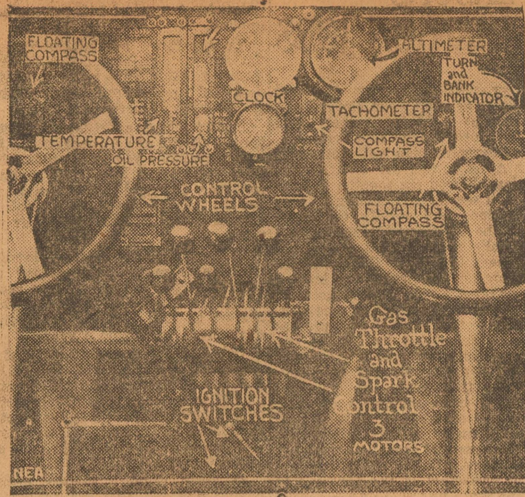
Here is the instrument board of the tri-motored Fokker monoplane, Bird of Paradise which Lieutenants Maitland and Hegenberger flew from San Francisco to Honolulu. Notice the spark and gas controls for the three motors.
