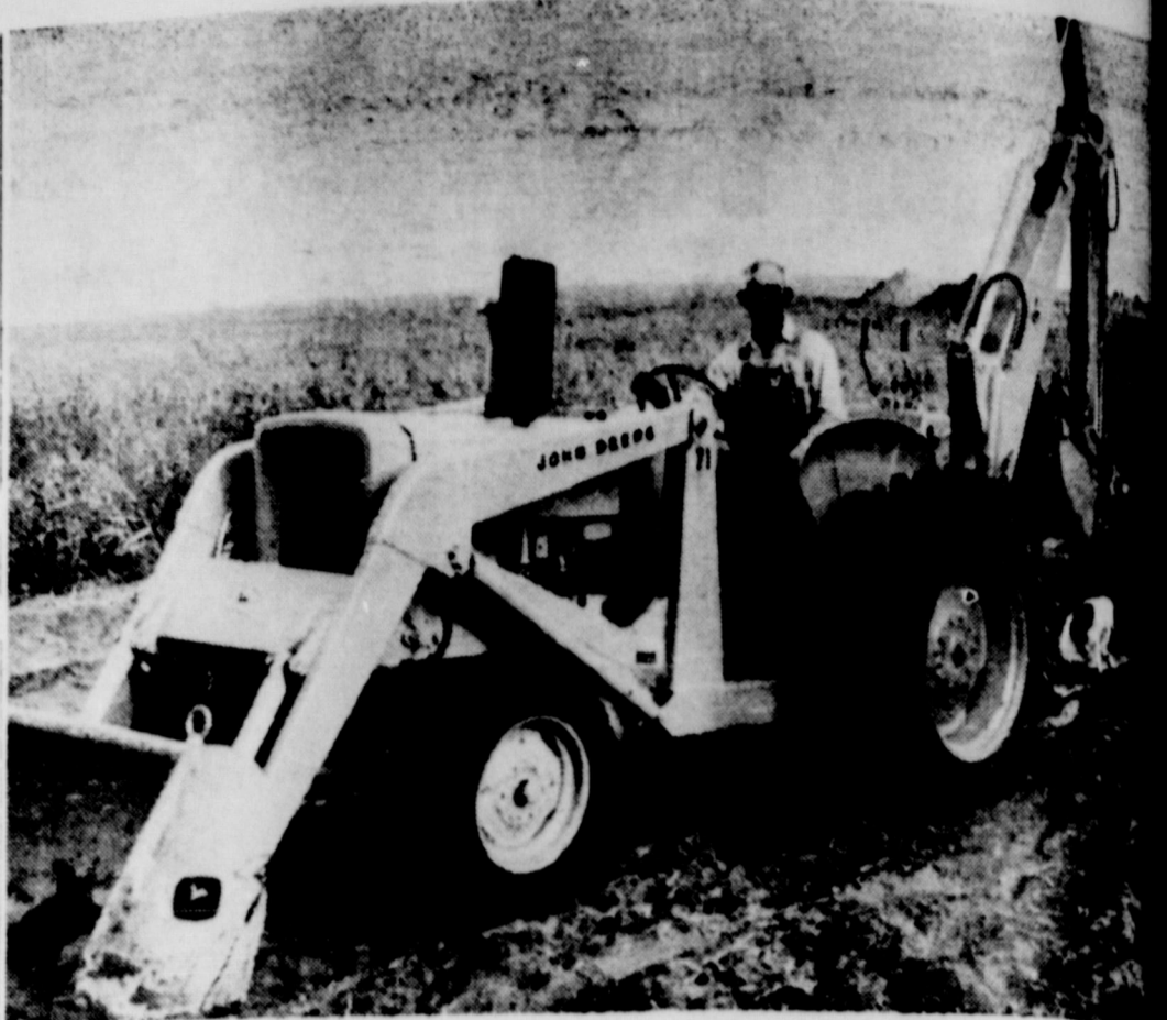
SOMETHING NEW FOR WHEELER: The above back-hoe-machine, owned by Rogers and Son of Wheeler, is one of the first to be located in this area. The big, intricate looking machine is capable of digging a hole 13 ft 6 inches deep. The machine which cost $7,000 will be used in the Wheeler area to dig cellars, septic-tanks, or any other type of dirt work.
