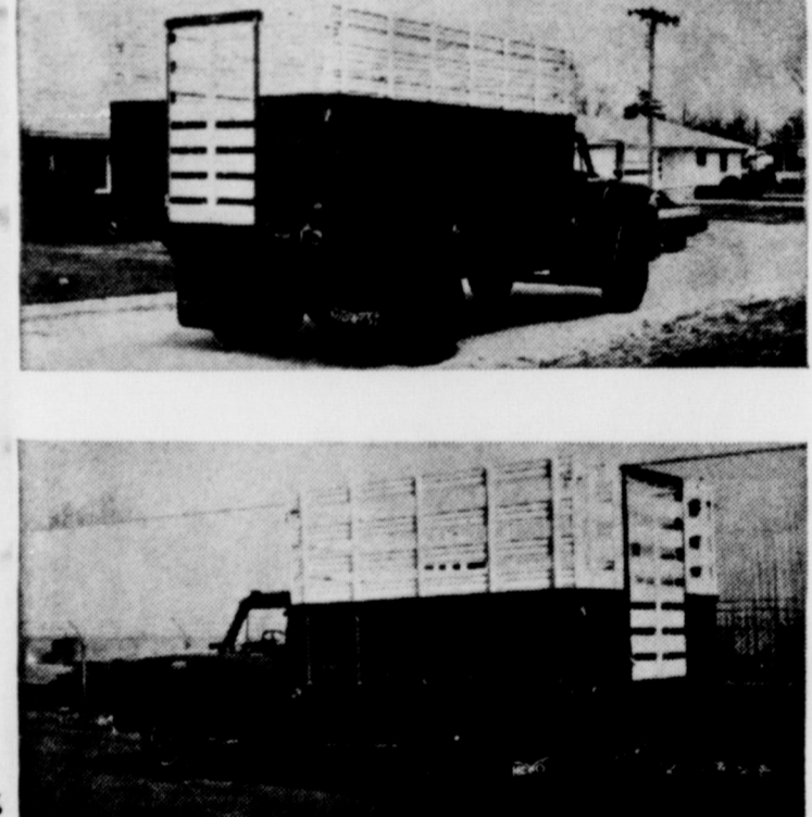
Two types of new steel stock racks have been developed by Mid West Body & Manufacturing Division, Paris, Ill. The 29-inch rack (top photo) fits on the 40-inch truck body. A 38-inch rack (bottom photo) fits on a 28-inch body.
