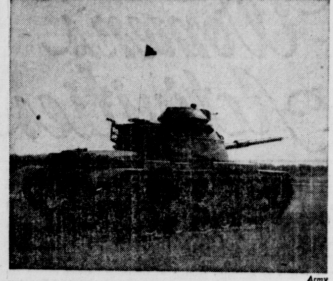
THE M-60 MAIN BATTLE TANK is the Army's newest and most powerful medium tank, mounting a 105mm gun capable of defeating all known enemy tanks, and a new 7.62mm machine gun, utilizing NATO ammunition. The tank's new Diesel engine is able to use several types of fuel and has greatly increased range. Chrysler Corp., Detroit, Mich., is prime contractor.
