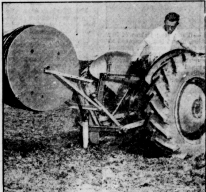
PIPE THIS—Farmer prepares to lay plastic pipe with this automatic device on a plot of land near Franklin, Pa., where the labor-saving mechanism is manufactured. Disposable reels holding up to 600 feet of piping are attached to the machine, which is constructed for a three-point hitch, but which is adaptable to any farm tractor, according to the manufacturer. Operating at tractor speed, it is designed to uncover a trench, lay pipe 14 to 20 inches deep and back-fill after itself, at the rate of 100 feet per minute.
