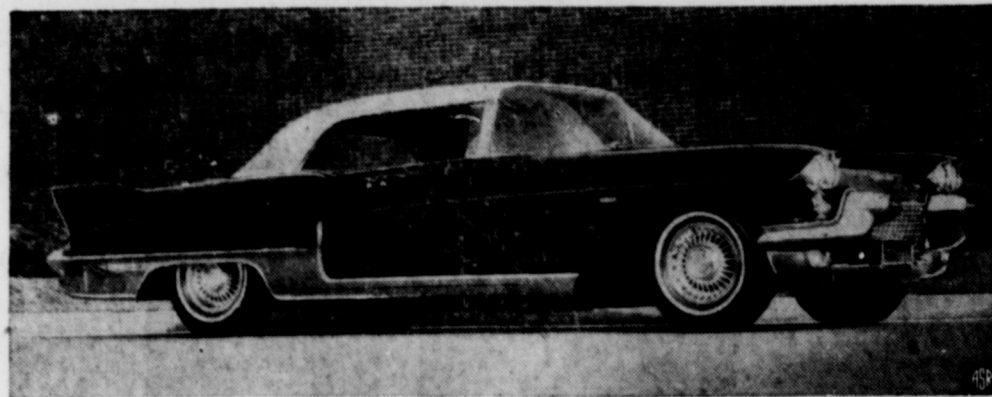
CADILLAC ELDORADO BROUGHAM —This new five-passenger super luxury sedan embodies many outstanding engineering and styling features never before incorporated on a production automobile. Completely modern in every detail, this distinctive four-door hardtop with a brushed stainless steel top has an extremely low over-all height of 55.5 inches. The first production model of the former Cadillac "dream car" will make its debut at the National Automobile Show in New York, December 8-15.
