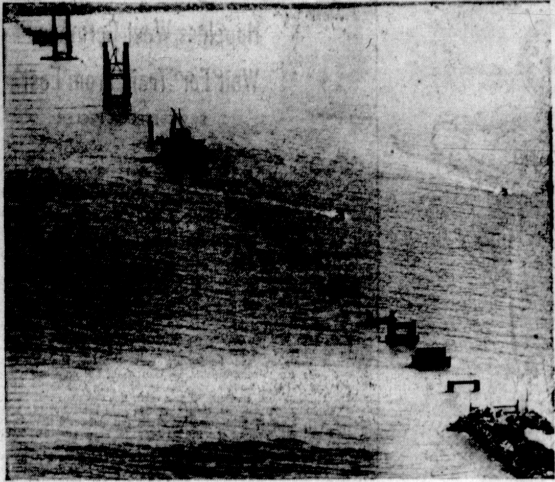
TWO YEARS TO GO —The 34 piers on which the 100-million-dollar Mackinac Bridge will rest stretch southward toward Mackinac City from the St. Ignace Causeway. The four-lane bridge will be 26,195 feet long, almost five miles. It will be the world's longest single-unit suspension bridge and should be completed in November, 1957.
