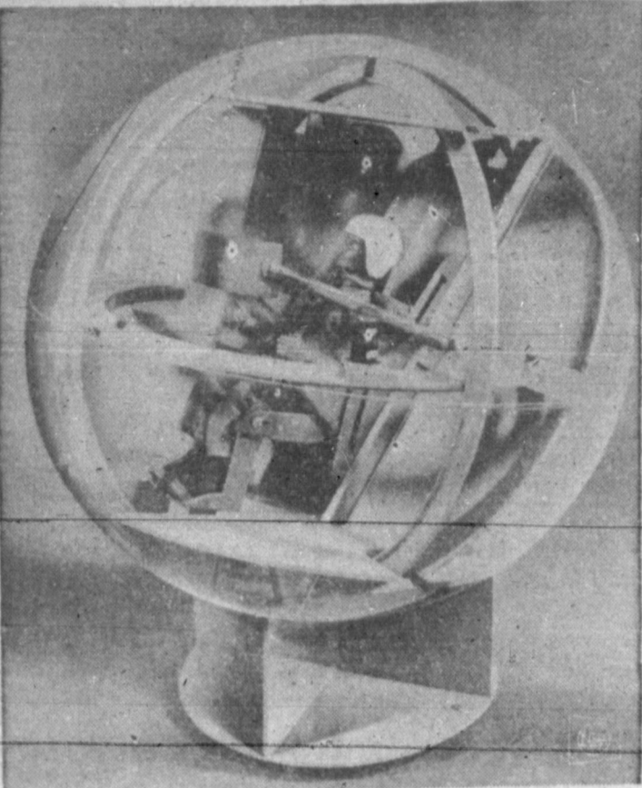
SPINNING MACHINE —The tumbling and spinning effects of a satellite in orbit will be studied by Air Force scientists in a simulator now under construction. Transparent model above shows the design of the unit, which will be a 10-foot-diameter glass fiber ball riding on a cushion of air. The motor-powered ball, under control of the pilot, will pitch, yaw and roll in all directions to test his physical and mental reactions. The simulator is being built by Norair Division of Northrop Corp. for the School of Aviation Medicine Brooks AFB, San Antonio, Tex.
