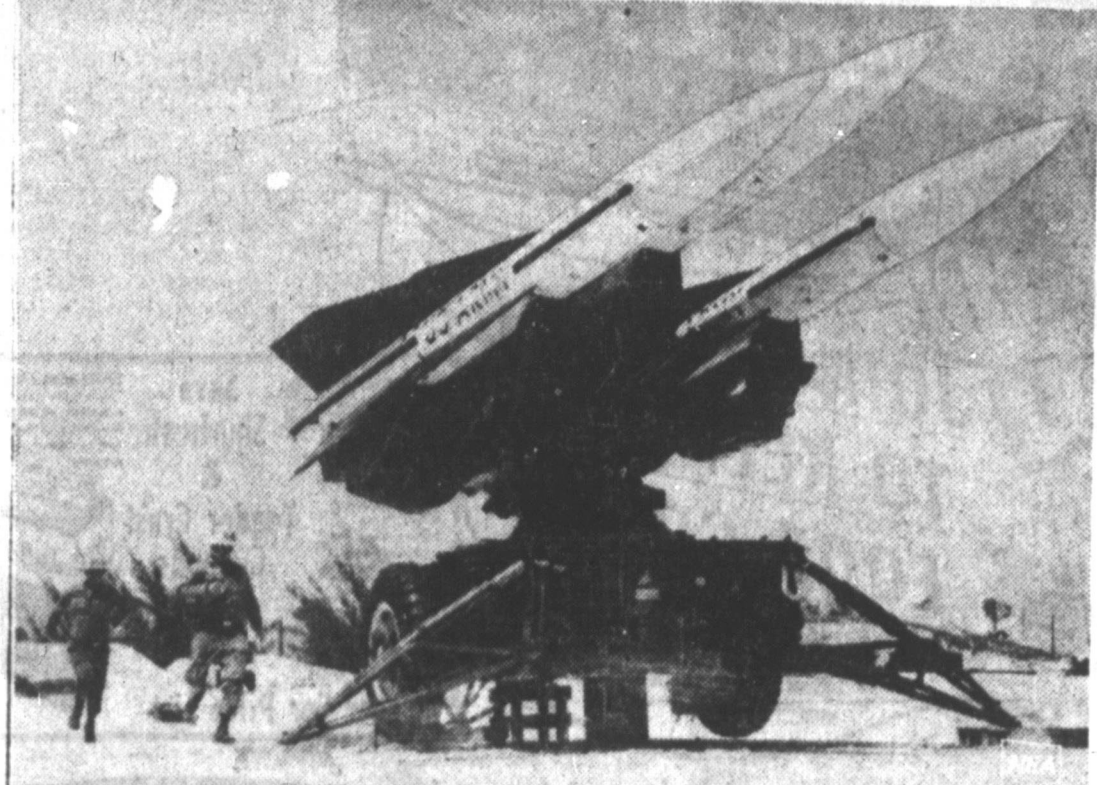
AIR DEFENSE —Hustling crewmen run to man an Army Hawk missile battery during a test drill in Florida. The mobile missiles were deployed on Florida's beaches during the Cuban crisis and have since become a permanent part of the Army Air Defense Command force.
