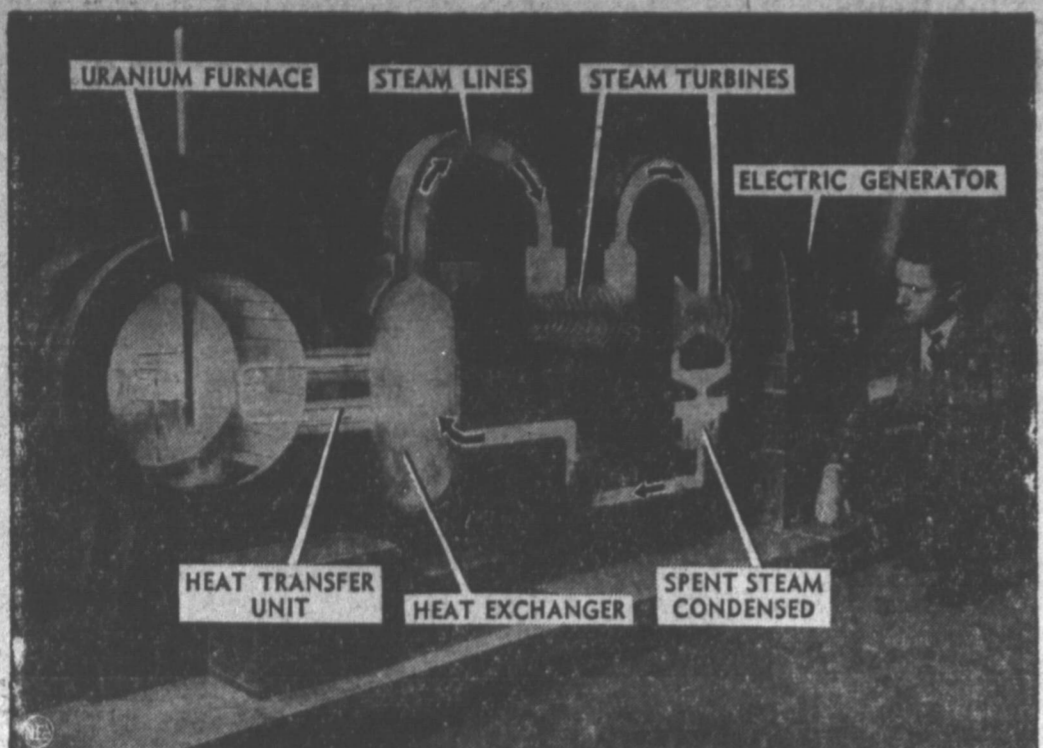
DESIGN FOR ATOMIC POWER —A simplified explanation of how the atomic power plant for the nation's first atom-powered sub will operate is offered by this model "mock-up," designed by Westinghouse, and placed on display in New York. When installed in the U.S.S. Nautilus, heat generated by splitting of the atom will be transmitted by fluid in a sealed, coiled pipe, to a "heat exchanger," or boiler. Steam will be formed in the water-filled boiler, pass through piping to the steam turbine, which will drive an electric generator to power the sub's electric motors. Spent steam will be condensed, pumped back to the heat exchanger. Demonstrating the power plant is Robert Dollison.
