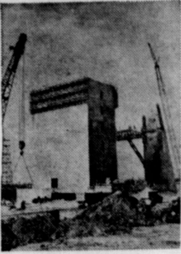
MOON 'SKYSCRAPER' . . . Stepping stone to the moon is this huge concrete and steel monolith under construction at the National Aeronautics and Space Administration (NASA) Saturn V test complex in Mississippi. Concrete forms of a special overlaid plywood are being stripped from the 102-foot level of what will be a test stand higher than a 20-story building.
