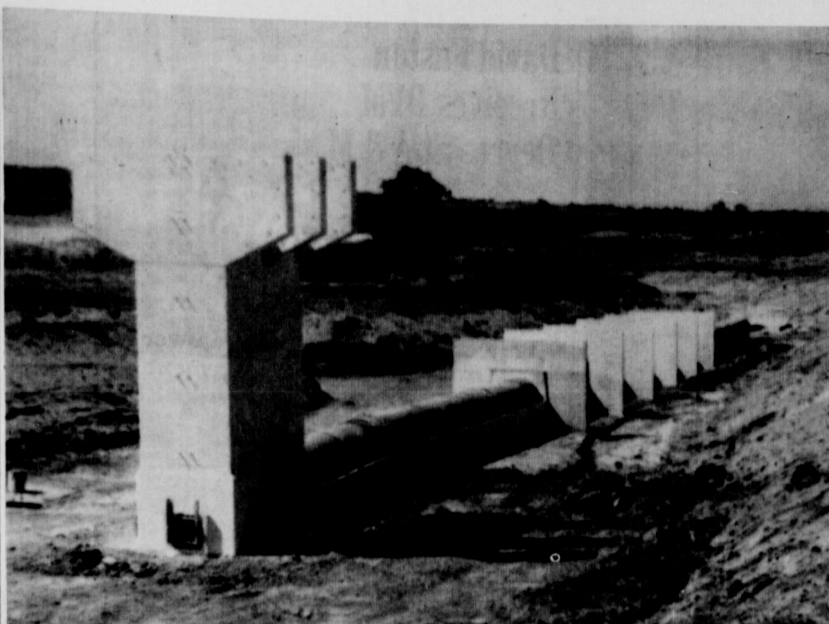
PRINCIPAL SPILLWAY —Pictured above is the 180-ft. long principal spillway at Site 5 of the Lakeview Watershed on a tributary of Bitter Creek. The dam is now under construction with the project about 50 per cent complete.
