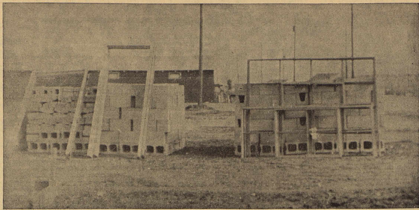
CONSTRUCTION IS NOW PROGRESSING on the new Cities Service Station here. The new station is inside the city limits, located on the Brownfield highway near Wagley's Garage. REVIEW Photo
