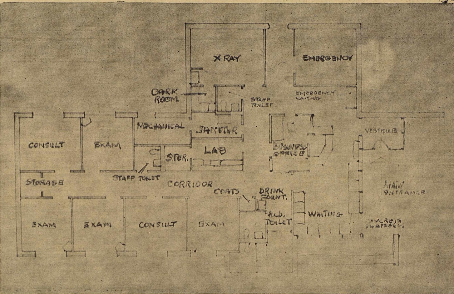
Floor Plan for Plains Clinic, Bids for Which Are to Be Let July 14
