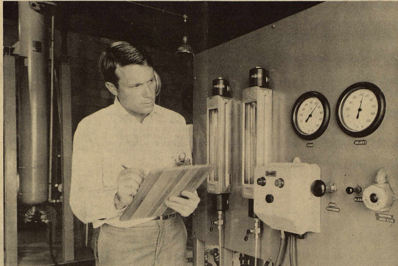
Field Test Engineer Daniel Crabbe makes routine inspection of control panel for Dupont's "Permasep" permeator undergoing tests at Foss reservoir near Clinton, Okla. Commercial size permeator, background, is also being used in brackish sulfate water tests at United States Public Health Service Hospital at Eagle Butte, S. D., and at Plains, Texas.
