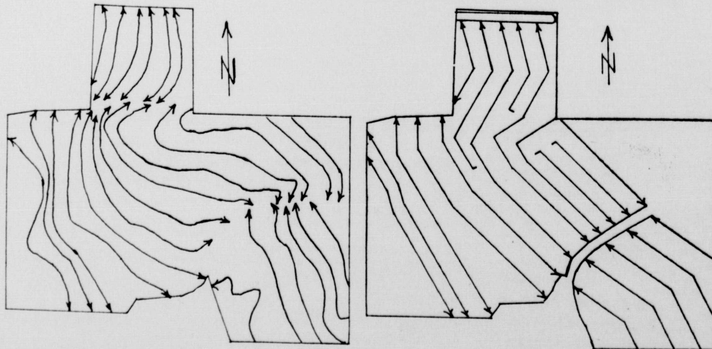
The two sketches above show advantages of a parallel terrace system over the conventional terrace system. The sketch on the left is the way Mr. McGinnis' terrace system looked before it was leveled and parallel terraces were constructed. The sketch on the right shows the new system of parallel terraces. The old conventional terrace system consisted of 57,120 feet. The new parallel terrace system consists of 38,544 feet.
