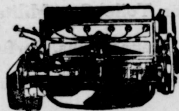
Chevrolet's new six-cylinder, fully enclosed valve-in-head engine has high compression non-detonating head. Its piston displacement is 194 cu. in. and it develops 46 H. P. at low engine speed.
