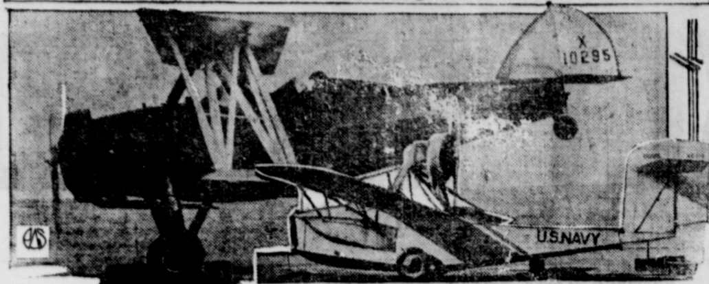
The large plane is the new invention of Albert Adams Merrill, which proved its ability to come to earth safely with the pilot's hand off the controls. The smaller is the new folding plane of the U. S. Navy, intended to be carried in an 8-foot tube on the deck of a submarine.
