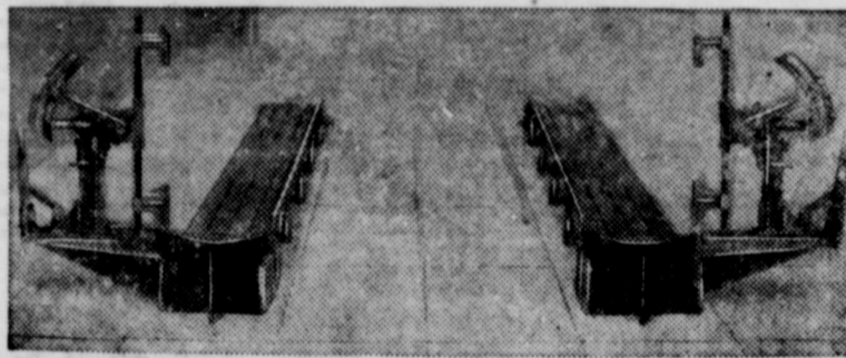
General View of Bean Wheel Aligning and Balancing Machine.
