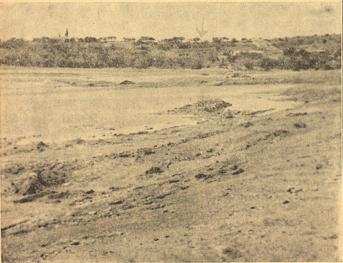
Site 13, on land owned by Bryan Hunt and George H. Neill, is shown holding some water at this early stage of construction. Note hospital in background. Ford Allen is the contractor, and contract cost is $45,206. Construction will be resumed in about two weeks, and the dam should be completed rapidly. Though Site 13 is on a small watershed (700 acres) a 10 to 20 inch rain could cause heavy damage to homes below. In addition, the construction of this dam helped get sufficient flood control to eliminate the necessity of widening Lowrey Draw through Sonora, which would have been much more expensive.
