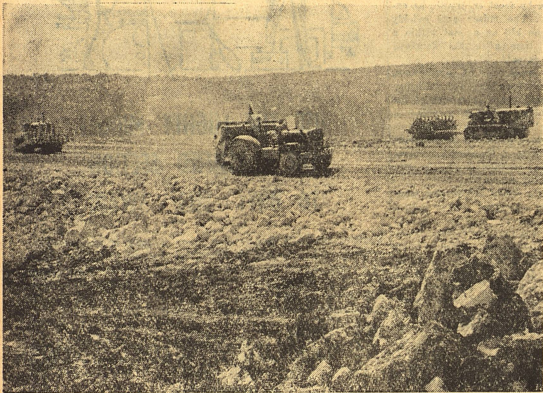
Site 12, on the W. A. Miers ranch near the Texas New Mexico Pipeline Station, lacks approximately 10 feet of its 35 foot height. Controlling floodwater from 4.38 square miles, this dam will hold 1,157 acre feet at emergency spillway level. Both sides of the structure will be blanketed with rock from the 150 foot rock spillway. Ford Allen is building this dam, and the contract cost is $73,664. It is expected to be completed in approximately two weeks.
