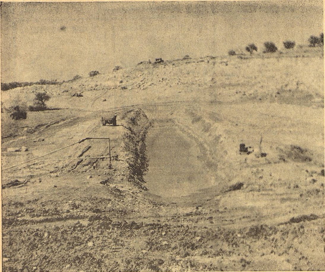
Site 11, on the W. A. Miers ranch 3 miles north of Sonora, showing the excavated core trench. This trench, dug 20 feet deep to insure a solid foundation for the dam and to reduce seepage, has filled twice from runoff water during the past 10 days. Three pumps can be seen draining the trench when the photo was taken. Site 11 will control floodwater from 17 sections of rangeland, and will detain 5,189 acre feet at emergency spillway level. The dam will be 47 feet high and contain 347,680 cubic yards of earth and rock fill. A 250 foot rock spillway can be seen in the background, and a 150 foot spillway will be constructed on the south end of the dam. Contract cost is $226,200 and R. L. McQuatters is building the structure for Cage Bros.
