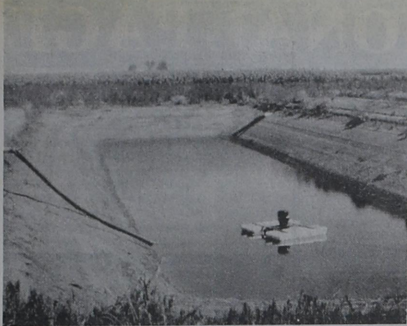
TAILWATER RETURN PIT...Many High Plains producers have constructed tailwater return pits to collect irrigation water that would otherwise be lost as tailwater. The collected water can then be pumped back onto the field for re-use.
