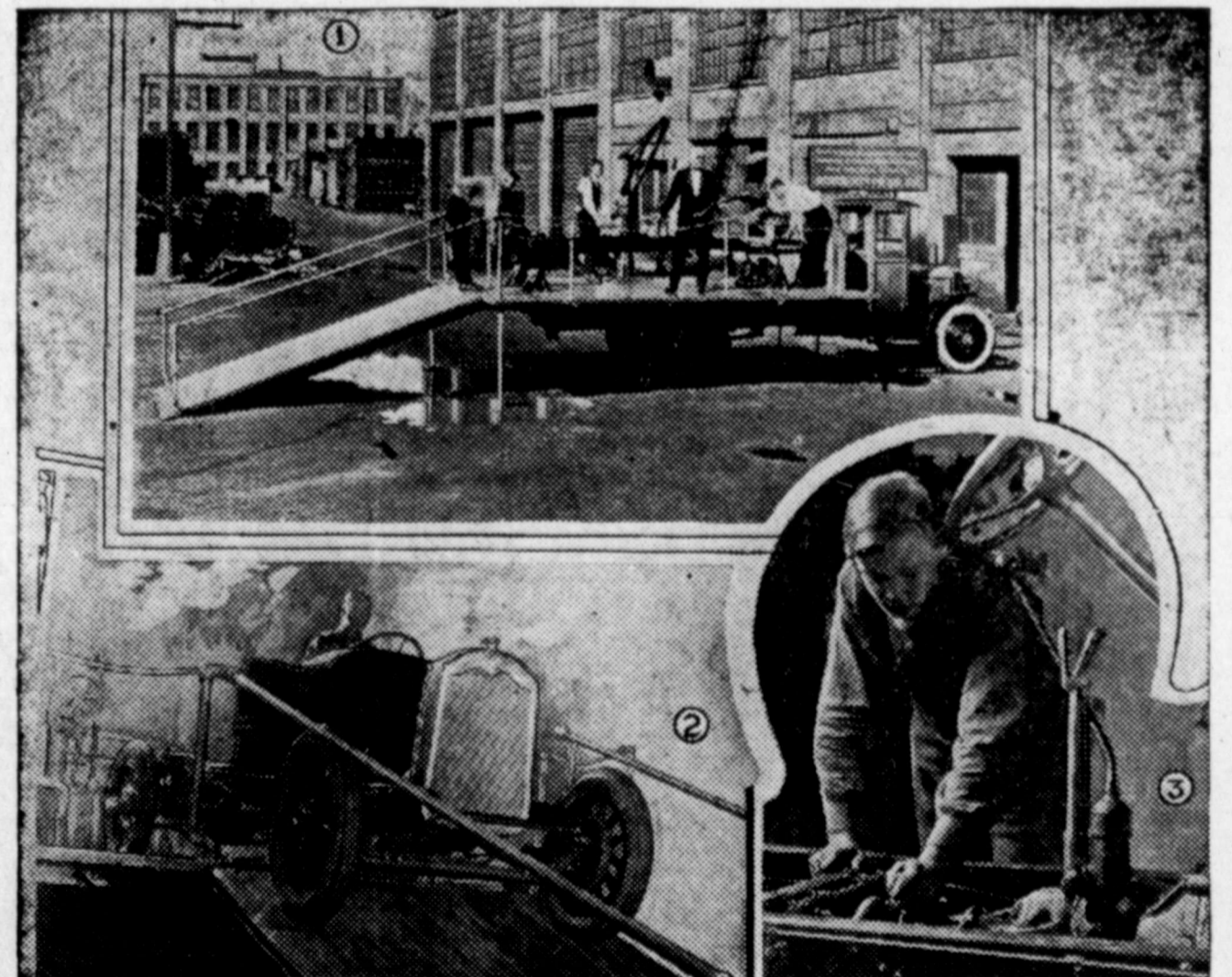
(1) Start of Assembly-Placing Frame. (2) Completed Chassis Being Driven From Platform. (3) Connecting Self-Lubricating Universal Joint to Torsion Tube.
