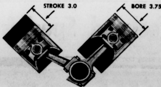
OVERSQUARE DESIGN is the mark of Chevrolet's modern truck V8's. The ultra-short stroke means less piston travel . . . less friction wear.
