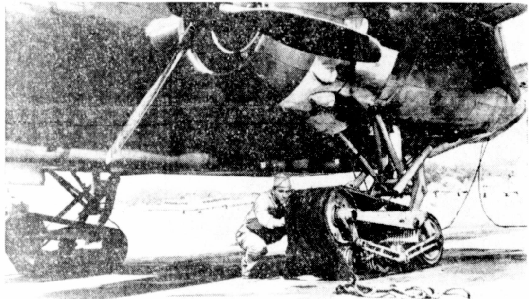
TO LAND ROUGHLY —Heavy planes can land safely on rough, soft or sandy terrain, with these miniature halt tracks for gear, up to speed of 120 miles an hour. U. S. Army Air Laboratory developed them with commercial firms.
