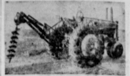
This posthole digger was built by Clyde Hall, Bradford, Ill. He says it will put a nine-inch hole down three feet in Illinois soil in three minutes. It was built of heavy materials in his farm shop and required some large welds. A car differential provides a way to use tractor power to dig postholes.
