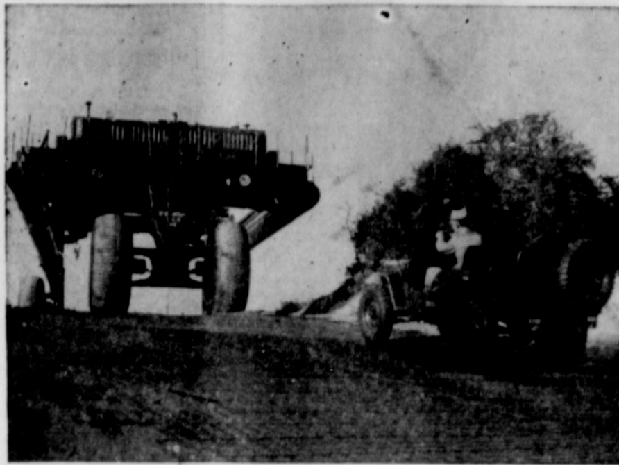
LIKE PRAYING MANTIS —The Army Transportation Corps' only Landing Craft Retriever looms ominously over a humble jeep at Fort Story, Va. The 181-ton LCR is actually very benign. It can wade into nine feet of water over a disabled or beached landing craft, tuck the 67-ton workhorse under its middle, and refloat it or tow it to the beach for repairs.
