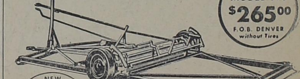
Width 12', Length 21' Cutting blade 9' 3" x 16" Weight 1450 lbs., 3 Plow Tractor
