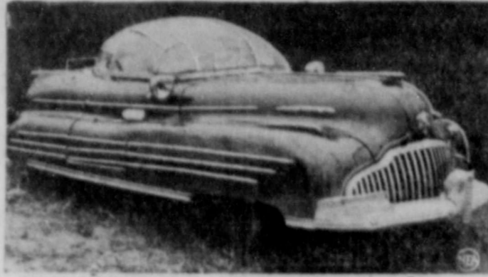
"Hollywood Streak" is the name given the auto above, designed by George Bartell, Detroit garage operator. Powered with a 100 hp. motor, it weighs 2200 pounds, is 48 inches high, 140 inches long and 60 inches wide. Top is transparent plastic.
