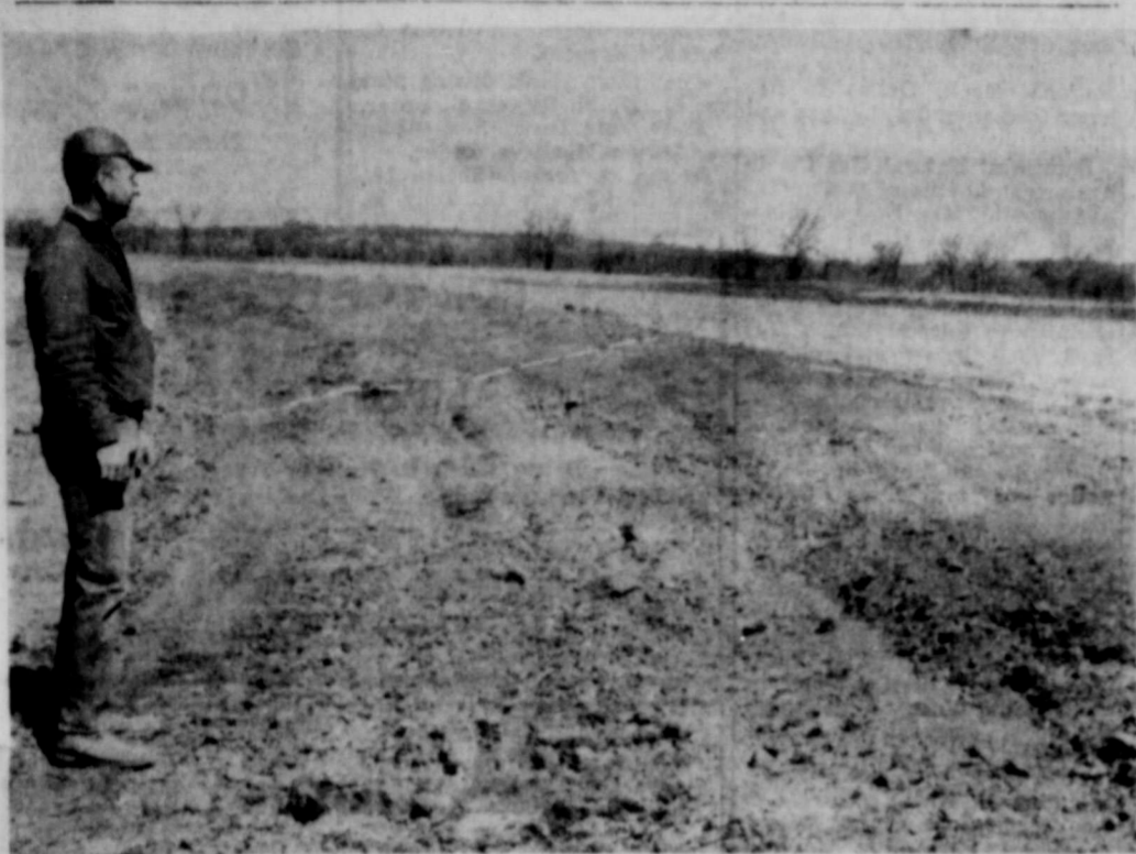
A good terrace is one which will carry a flood and yet be easily farmed. Terraces inspected here by Paul Norris on his farm northeast of Carbon, are an example of terraces with a big water capacity and smooth flat side slopes adapted to modern farming equipment. Steps in the construction of these terraces are shown in the lower photos.
