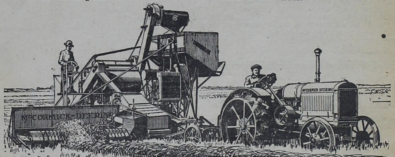
McCormick-Deering No. 11 Harvester-Thresher with 6½-foot pick-up device, handling the grain from a 16-foot swath cut by windrow-harvester
