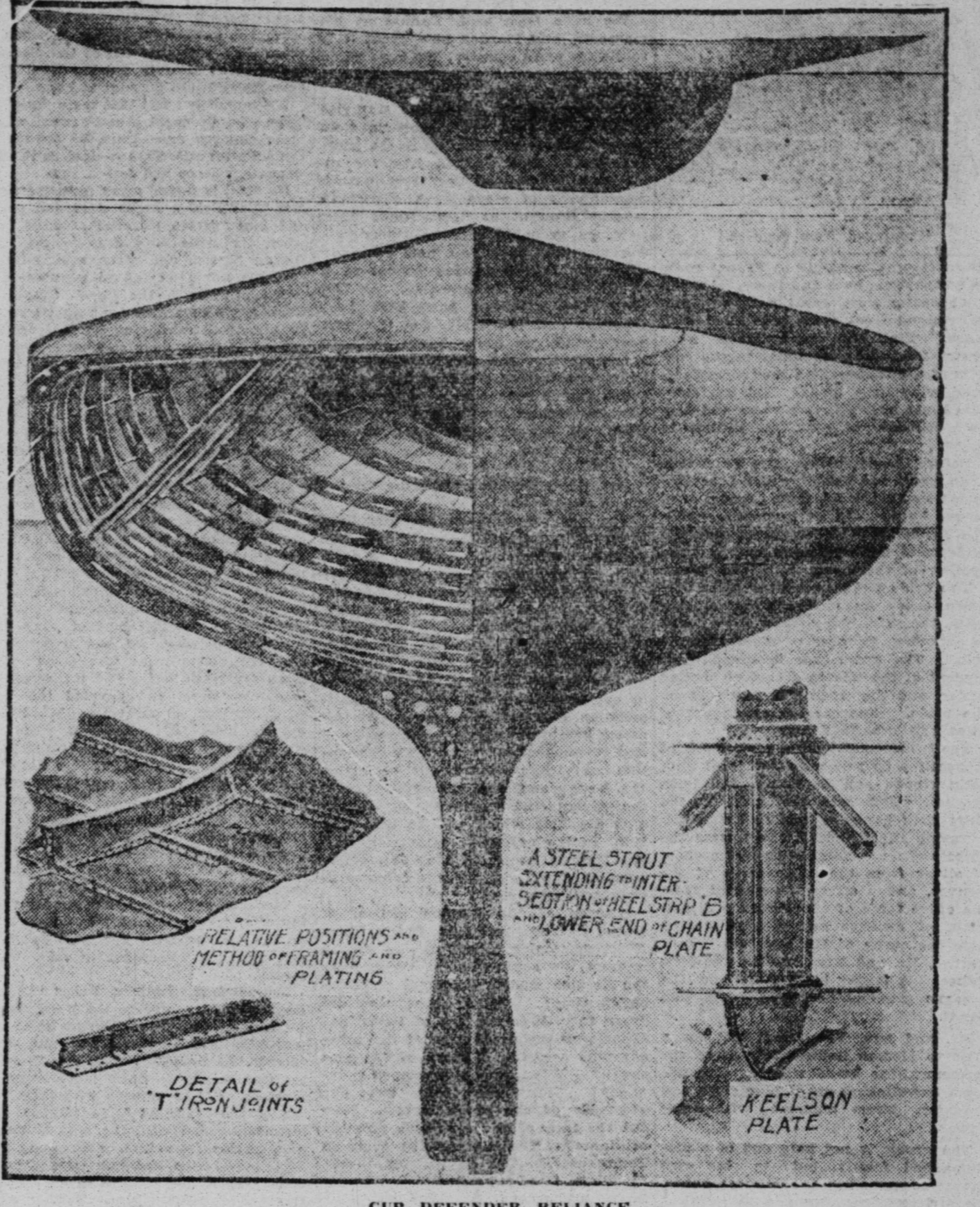
CUP DEFENDER RELIANCE (Copyright, 1903, by W. R. Hearst) The picture shows the details of the construction of the American cup defender, Reliance. It shows the fullness of her midship section and her scow finitype. The belt and longitudinal framing of the Constitution has been adopted with practically no change in the new defender.
