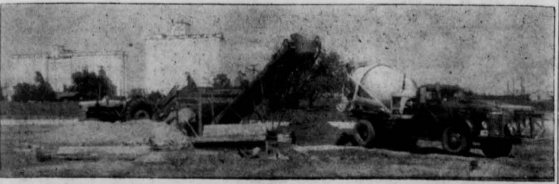
THIS IS THE equipment of Dimmitt Ready-Mix, a new concrete mixing firm which began operations in Dimmitt this week. It is located at East Second and Stinson Streets.
