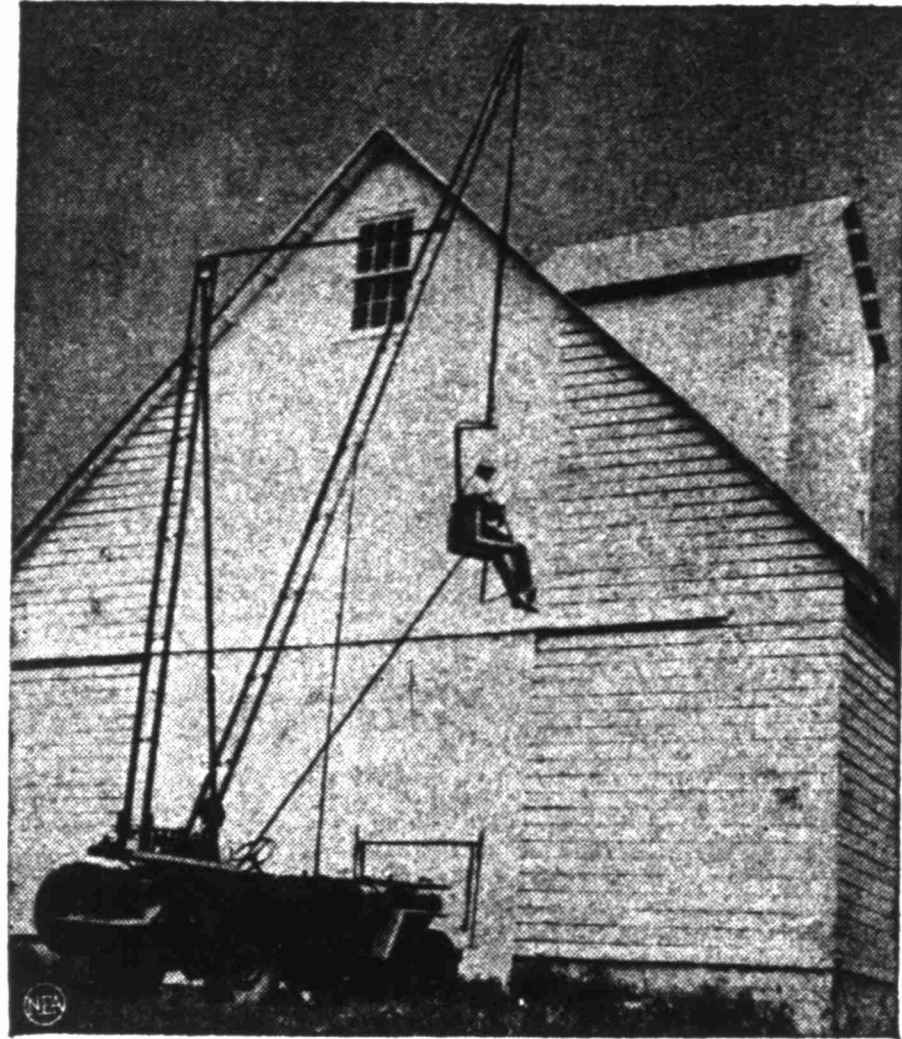
A spray-painting service in Lincoln, Ill., is throwing its ladders and scaffolding right out the window. It developed this aerial telescope boom that eliminates such paraphernalia. Mounted on a jeep, the 35-foot device makes painting this barn a one-man job.
