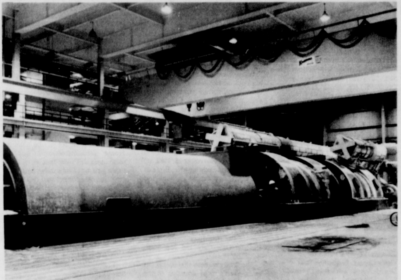
OPEN HOUSE SET.... Shown is one of the enormous turbine generators at Southwestern Public Service Company's Muleshoe plant. The generator can produce 561,000 kilowatts, enough electricity for 225,000 people. Open house for the new electric plant is scheduled this weekend.
