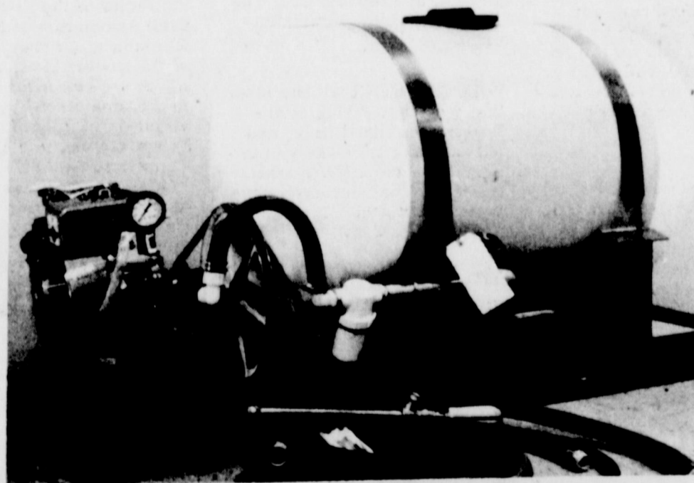
MODEL 1000 HYPRO POWER SPRAYER AS ABOVE BUT ALSO
