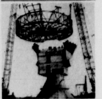
CAREFUL . . . The 35-ton steel framework of the "dish" of a new radio telescope is lifted in one piece and placed in position at Chilbolton, England. The "dish" is 82½ feet in diameter.
