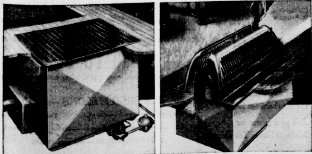
1. Coleman Gas Flat-Register Models sit in floors, no basement needed. Sizes for 2 to 5 Rooms—25,000 to 70,000 BTU. 2. Coleman Duel-Wall Model. Set under wall, use no floor space. 25,000 to 70,000 BTU.
