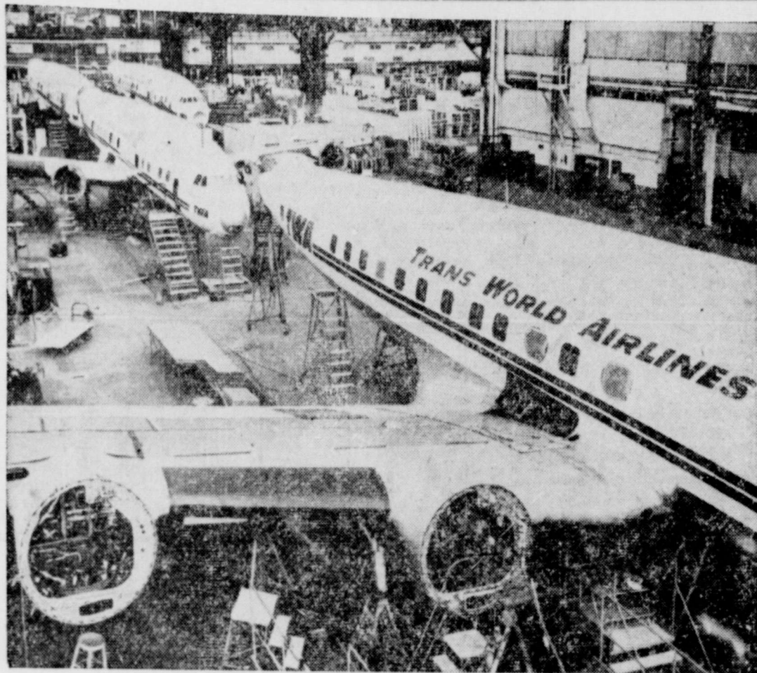
NEW AIRLINER STYLE—Fuselages of redesigned Super Constellation transports are receiving tail structures, wings, landing gear and engines on an assembly line in Burbank, Calif. The planes are powered by 10,400 horsepower and will be used for transcontinental service.
