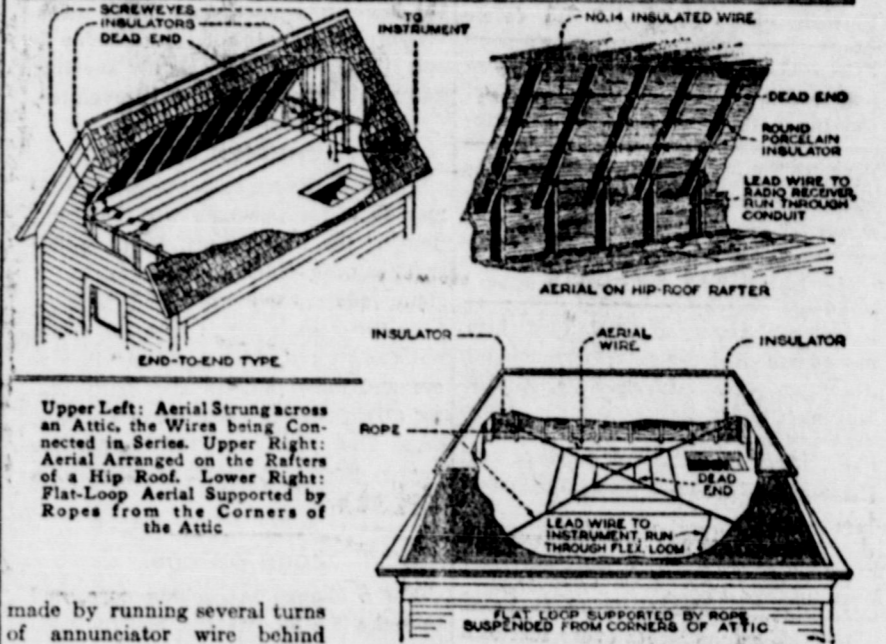
Upper Left: Aerial Strung across an Attic, the Wires being Connected in Series. Upper Right: Aerial Arranged on the Rafters of a Hip Roof. Lower Right: Flat-Loop Aerial Supported by Ropes from the Corners of the Attic.
