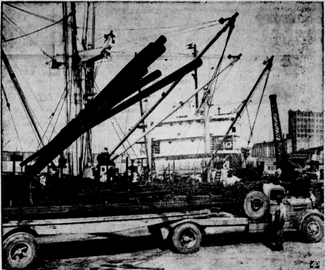
PIPES FOR TEXAS OIL FIELD A portion of a 4900 ton shipment of oil pipe is unloaded at a Houston dock for use in Texas oil fields, where a critical shortage exists, after it is straightened. The pipe came from the dismantled Canol pipe line, wartime Canadian project undertaken by the U. S. government. (AP) Photo
