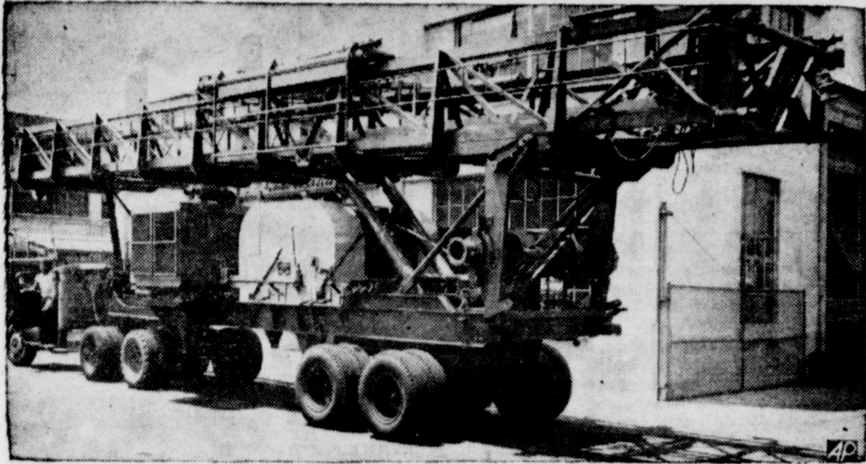
THE NEW LOOK—IN RIGS First of the new type, hydraulically raised, mobile telescope rigs to be used in West Texas, has been put in operation east of Blair in Taylor county by
