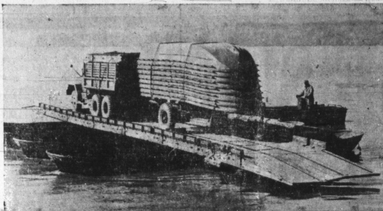
RAFT —New lightweight raft developed by the U.S. Army Engineer Research and Development laboratories, Fort Belvoir, Va., carries a truck and trailer loaded with components that comprise the ferry. Propelling the raft is a 19-foot power boat. The raft can carry 12-ton loads in currents as swift as eight feet per second. Heaviest component is a 650-lb. ponton.
