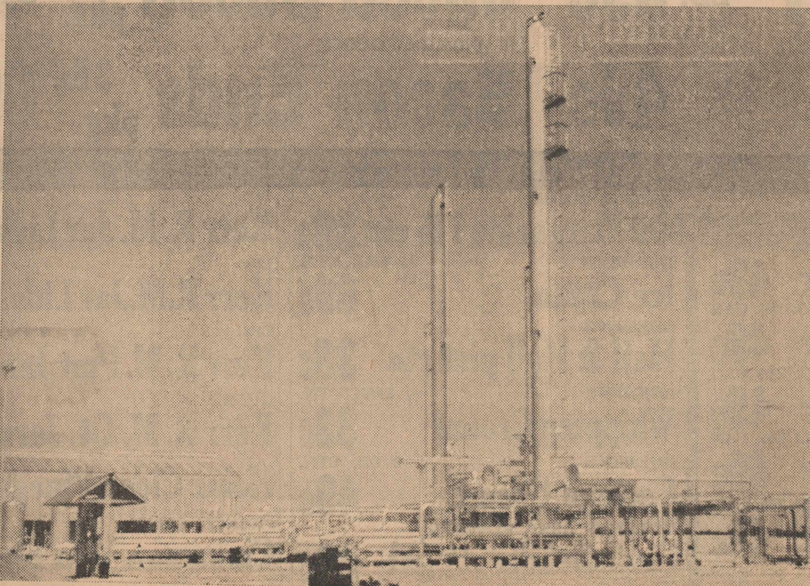
AN OVERALL VIEW of the process area shows the deethanizer and debutanizer fractionating columns with their accessory exchangers, pumps and vessels, the compressor building, left background and the electrical switchgear, left.
