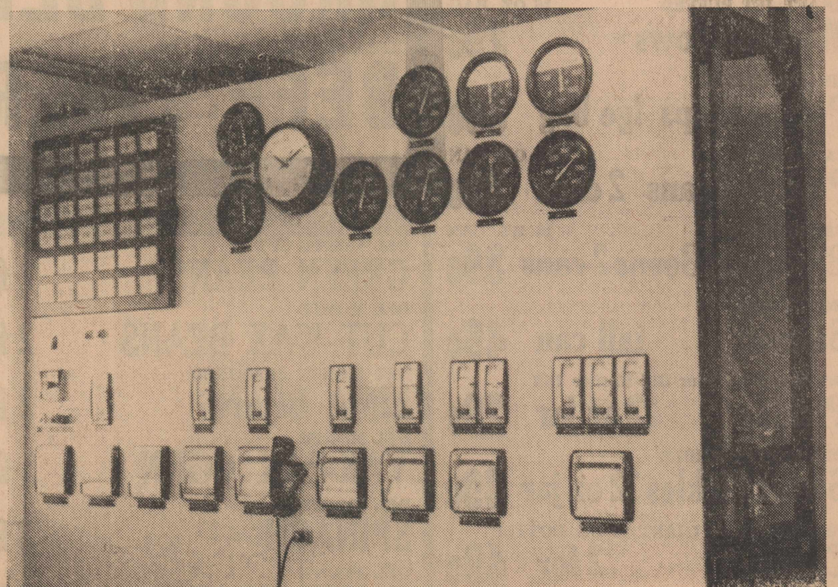
CENTRAL CONTROL PANEL has controls for various process variables, the alarm annunciator panel and pressure gauges which show compressor discharge pressures. The entire plant process can be supervised from this point.
