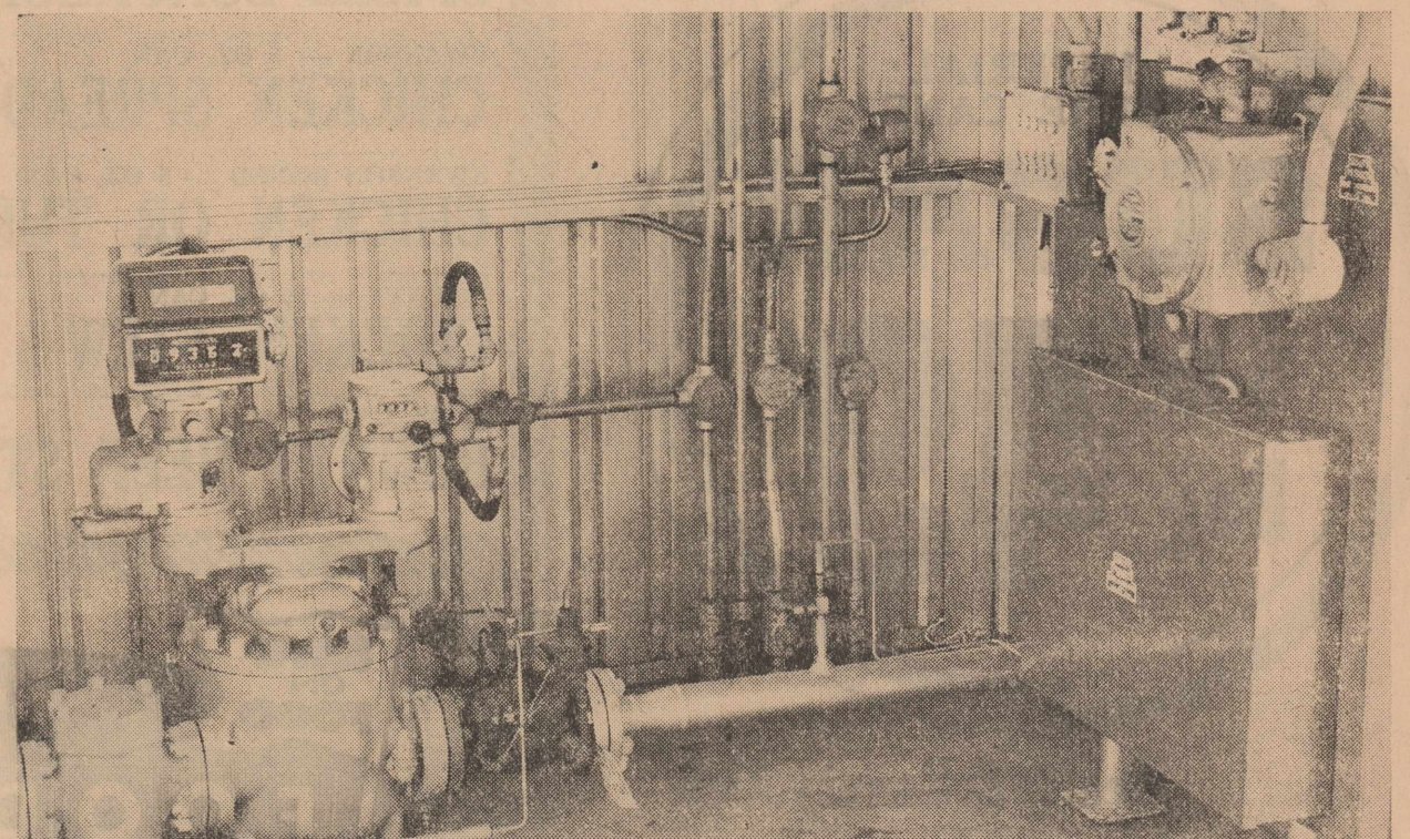
HELP YOURSELF meter and control equipment, shown here, permits driver attended loading of LPG production. Numerous shutdowns are provided to assure a safe loading operation.
